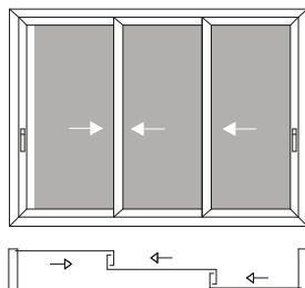
5A 3 vie - 3 ante 3 rail-3 sash
