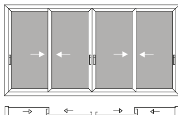
7A 2 vie - 4 ante 2 rail-4 sash
