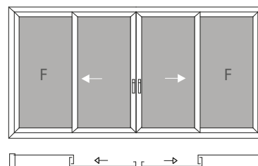
8A 2 vie - 2 ante+2 fissi 2 rail-2 sash+2 fixed
