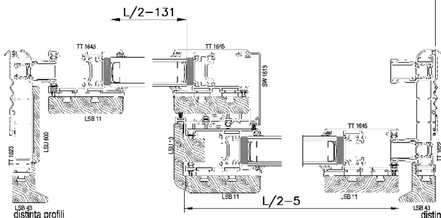
LSB 43 distinta profili
